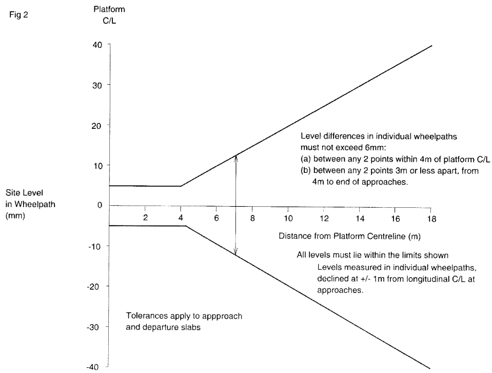
EMU SITE LEVEL TOLERANCES
