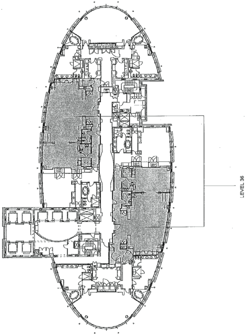
PLAN 4 MAIN CASINO - LEVEL 36 DECLARED SMOKING AREAS
